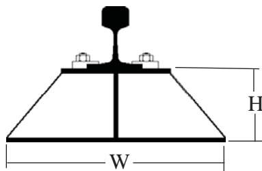
Type TN 150
