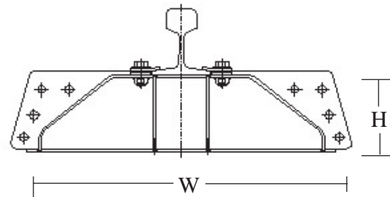
Type TN 406
